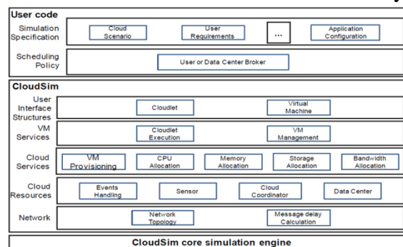
Fig. CloudSim Architecture
