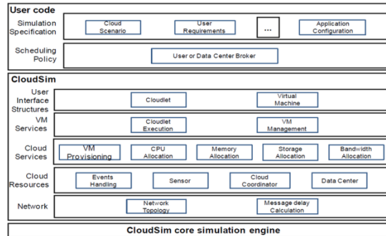
Fig. CloudSim Architecture
