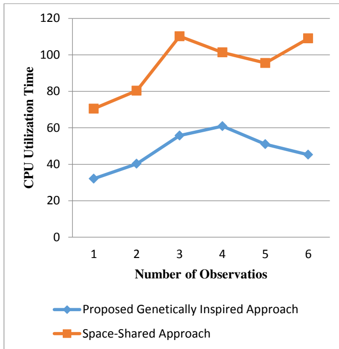
Figure 4.1: Comparative CPU utilization
